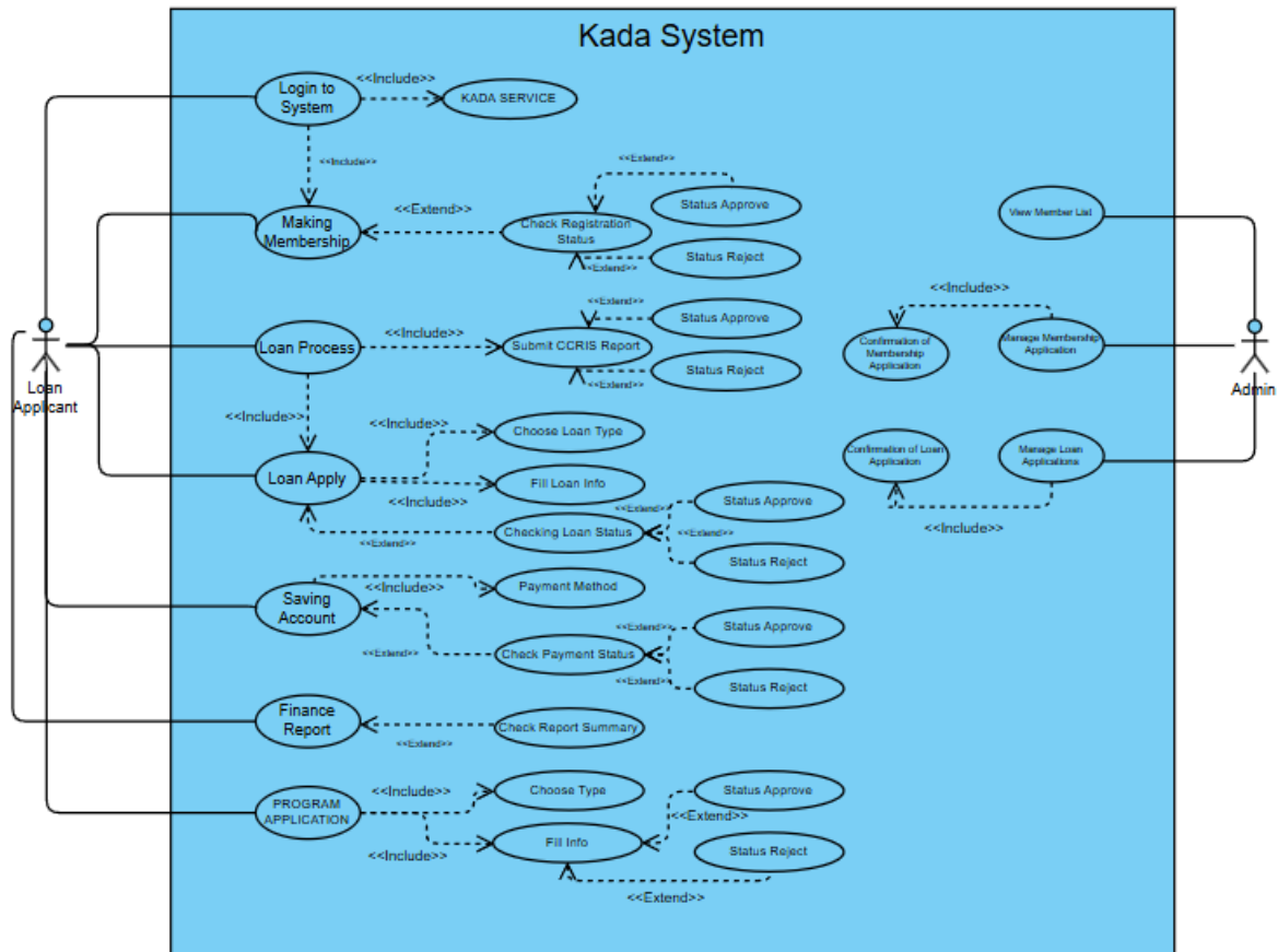
Figure 5: Use Case Diagram for KADA System
